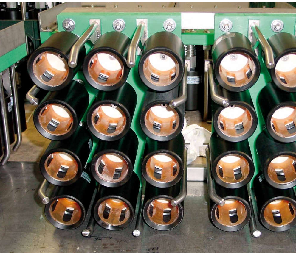
Special manual packing head for repacking 2 six-pack packages in pinole box
