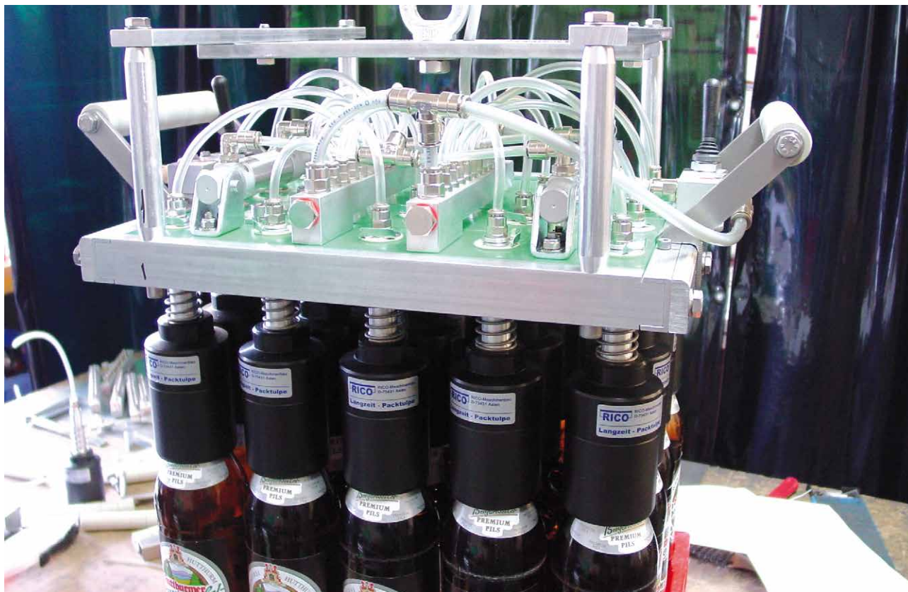
Manual packing head with 20 gripper heads for 0,5 l Euro bottles
